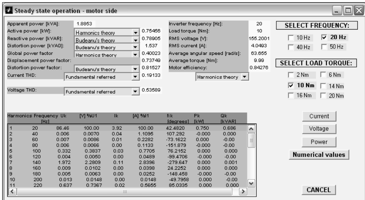
Figure 15: The Numerical values window – the motor side at 20Hz and 10Nm.
