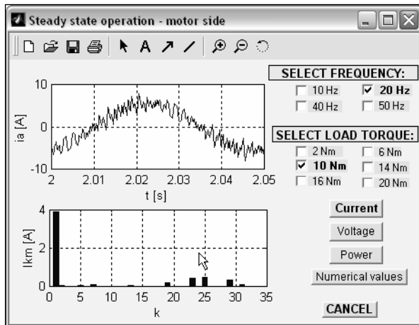
Figure 14: The load current and its harmonics spectra
