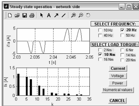
Figure 10: The network current and its harmonics spectra
