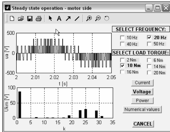
Figure 13: The output phase voltage and its harmonics spectra
