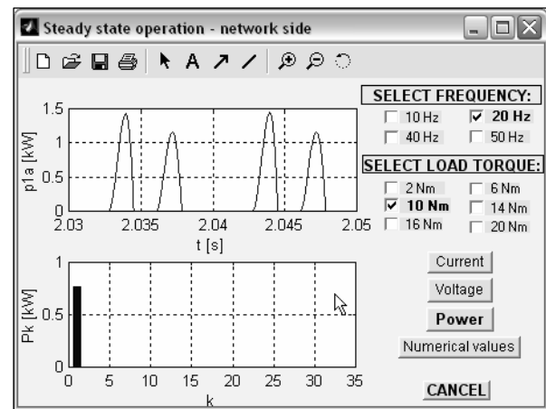
Figure 11: The network instantaneous power and its harmonics spectra
