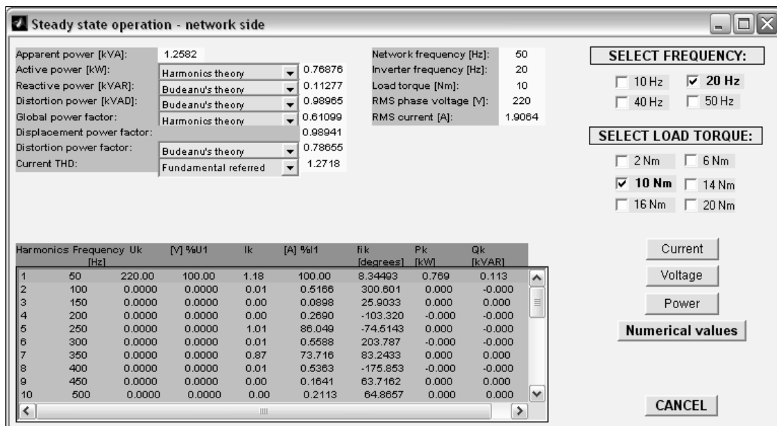
Figure 12: The Numerical values window – the network side at 20Hz and 10Nm.
