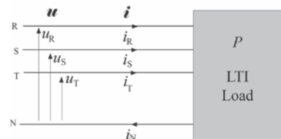
Fig. 5. Three-phase LTI load supplied in a system with neutral conductor.
