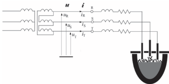
Fig. 2. AC arc furnace and its supply structure.
