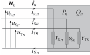
Fig. 6. An equivalent circuit of the load for the n^{\text{th}} order harmonic.
