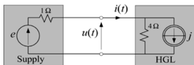
Fig. 7. Circuit with harmonic generating load (HGL).
