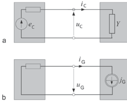
Fig. 9. (a) Equivalent circuit for harmonics n \in N_C (b) equivalent circuit for harmonics n \in N_G .
