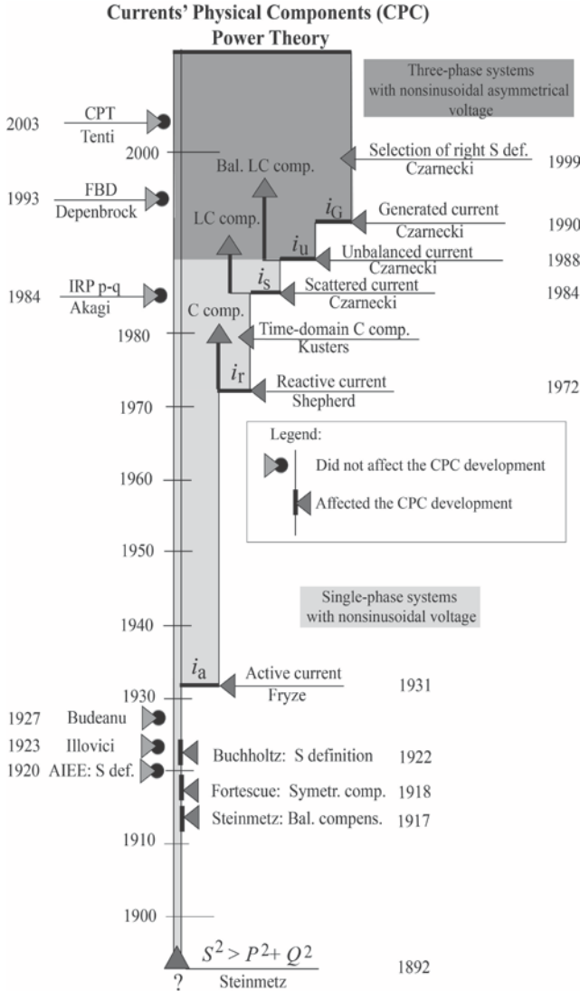
Fig. 4. Diagram which illustrates the development of the CPC-based power theory.
