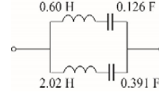
Fig. 6. Structure and parameters of a compensator branch.
