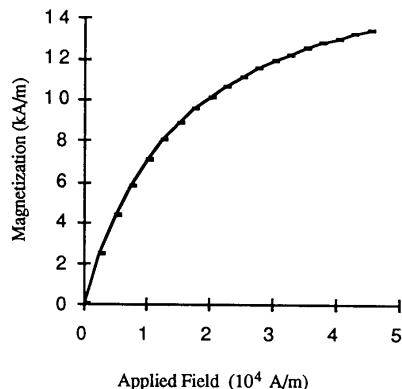
Fig. 1. Magnetization as a function of applied field.
